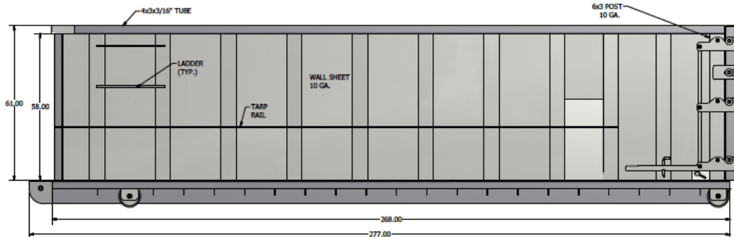
LATCH SIDE VIEW
