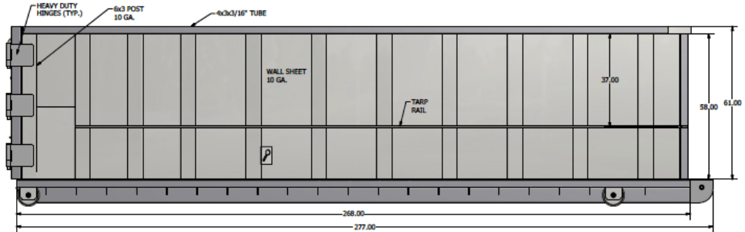
LATCH SIDE VIEW
